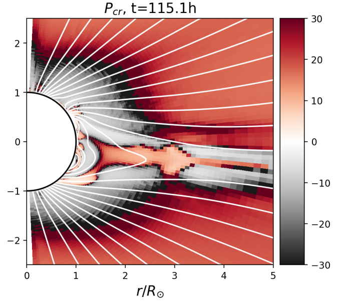
Fig. 9. Period of the pressure driven instability in the close corona. The panel shows a meridional cut at \phi = \pi ( 180^{\circ} longitude) for the June 14 simulation. Grey regions mark stable zones. In the inner corona, we clearly identify the tip of helmet streamers and the HCS as unstable zones, with typical P_{cr} \sim 10 - 30 hours.
