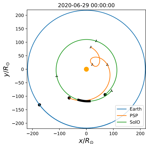
Fig. 1. Relative positions of PSP and Solar Orbiter in the solar Carrington frame on June 29, 2020. The back traced trajectory goes back to May 27 and ticks indicate the positions of the spacecraft every 11 days (the whole interval represents 33 days). The thick black line corresponds to available measurements of SWA/PAS.
